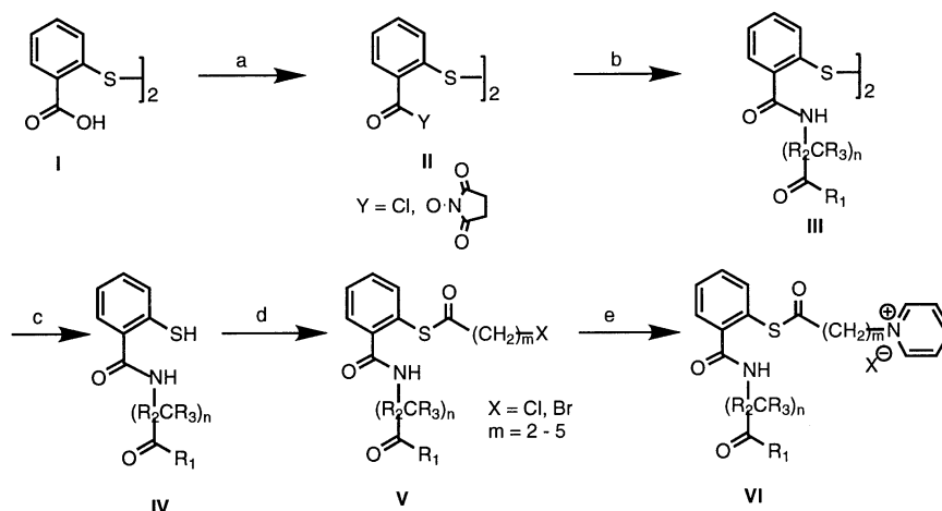
Scheme 1. Reagents and conditions: (a) \text{SOCl}_2 , 80^\circ\text{C} or N -hydroxysuccinimide, DIC, THF-2-PrOH, 25^\circ\text{C} ; (b) \text{H}_2\text{N}(\text{CR}_2\text{R}_3)_n\text{COR}_1\cdot\text{HCl} , 4-methylmorpholine, DMA, 0^\circ\text{C} or \text{H}_2\text{N}(\text{CR}_2\text{R}_3)_n\text{COR}_1\cdot\text{HCl} , \text{Et}_3\text{N} , DMF, 25^\circ\text{C} ; (c) TCEP·HCl, \text{Et}_3\text{N} , DMF/ \text{H}_2\text{O} (9:1), 25^\circ\text{C} ; (d) \text{ClCO}(\text{CH}_2)_m\text{X} , DMA, 25^\circ\text{C} ; (e) pyridine, under \text{N}_2 , 25^\circ\text{C} .
